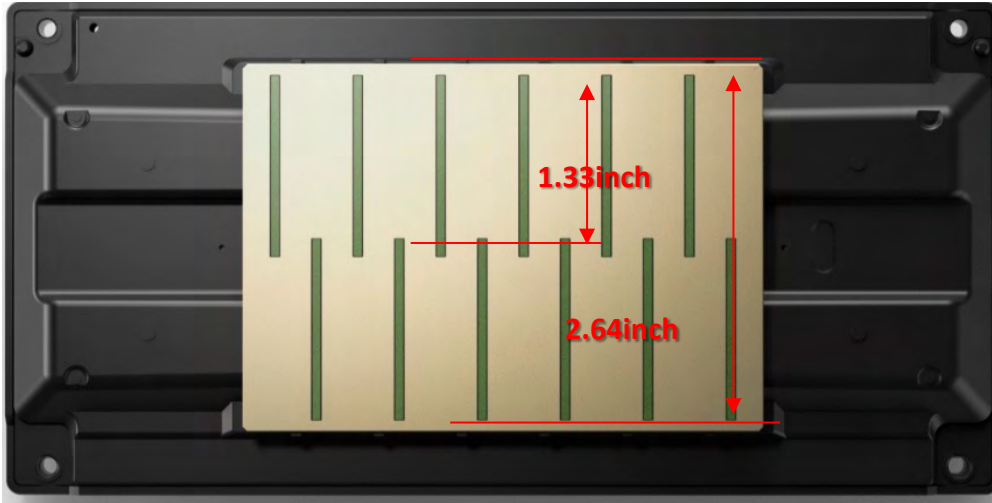
PrecisionCore MicroTFP 12 chip printhead
